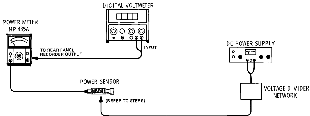
Figure 4-2. Instrumentation Accuracy Test Setup Without Calibrator
