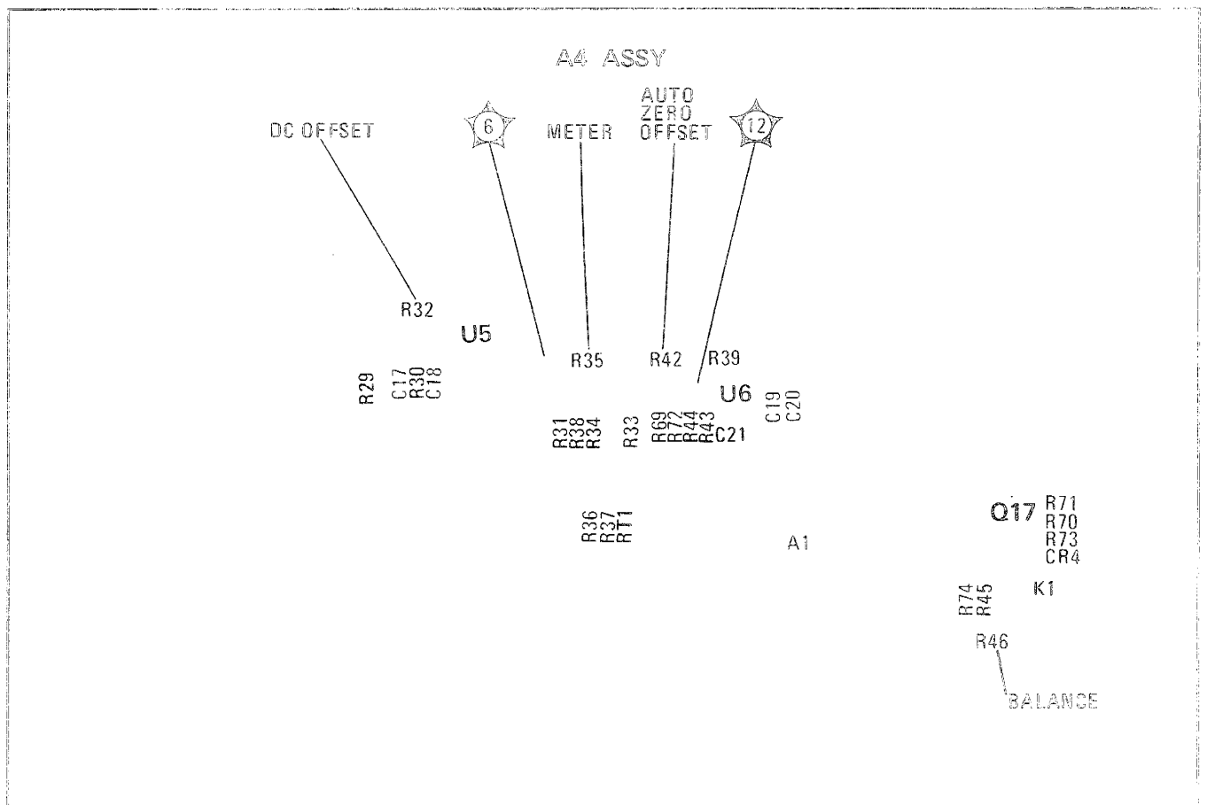
Figure 8-10. P/C A4 Assembly (DC Amp/Auto Zero) Components and Test Point Locations
