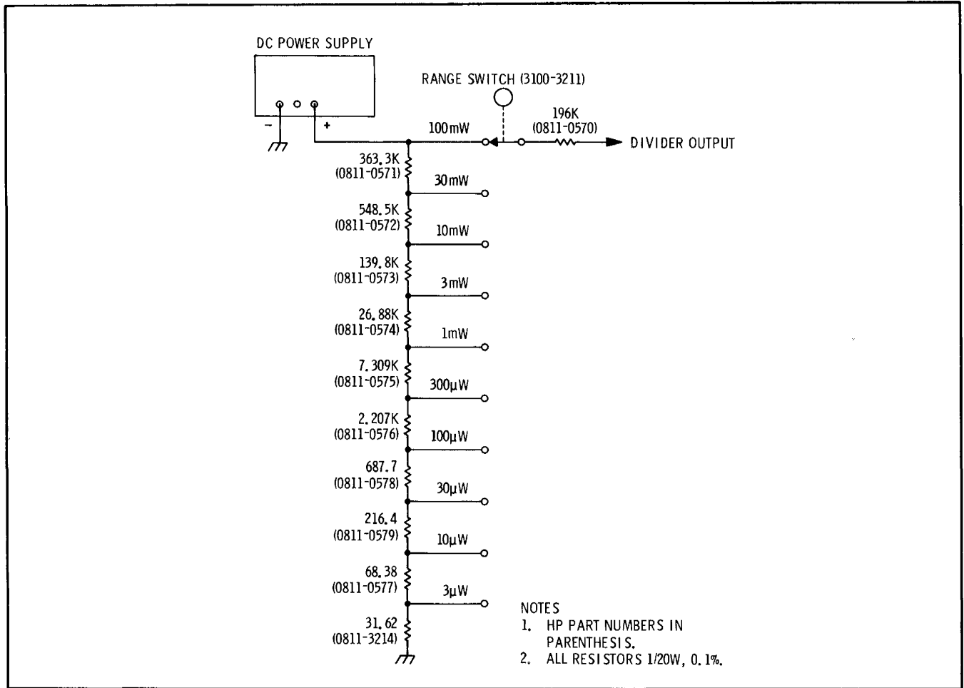
Figure 1-2. Voltage Divider Network
