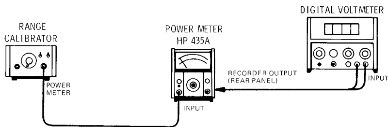
Figure 5-2. 435A Adjustment Setup With Calibrator
