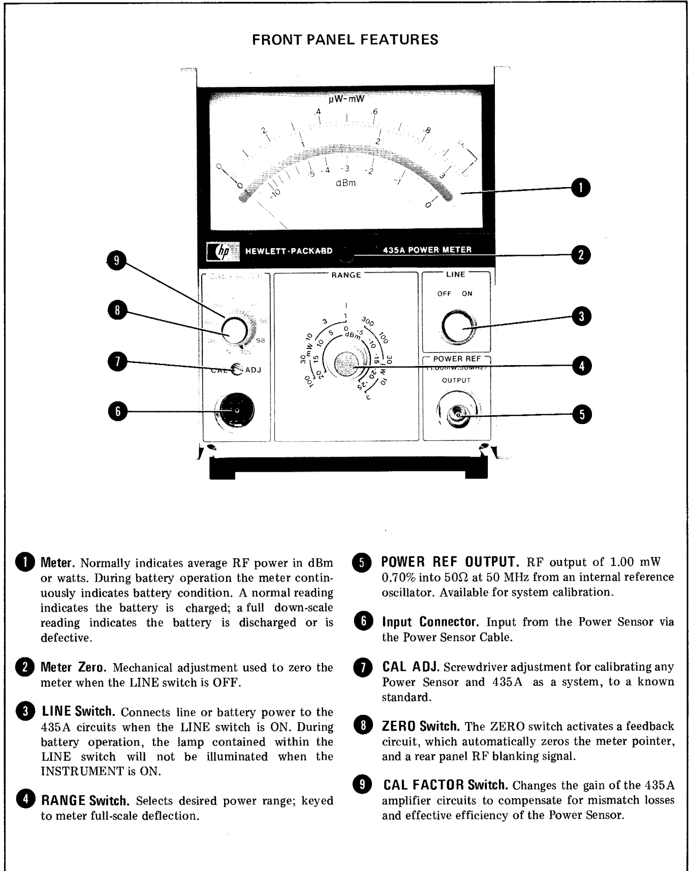
Figure 3-2. Front Panel Controls, Connectors, and Indicators
