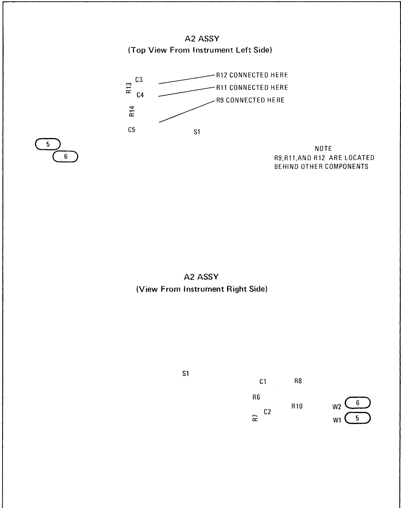
Figure 8-8. A2 RANGE Switch Assembly (Low Pass Filters) Component Locations
