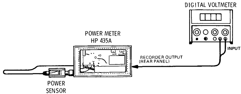
Figure 5-1. Power Meter Adjustment Setup without Calibrator
