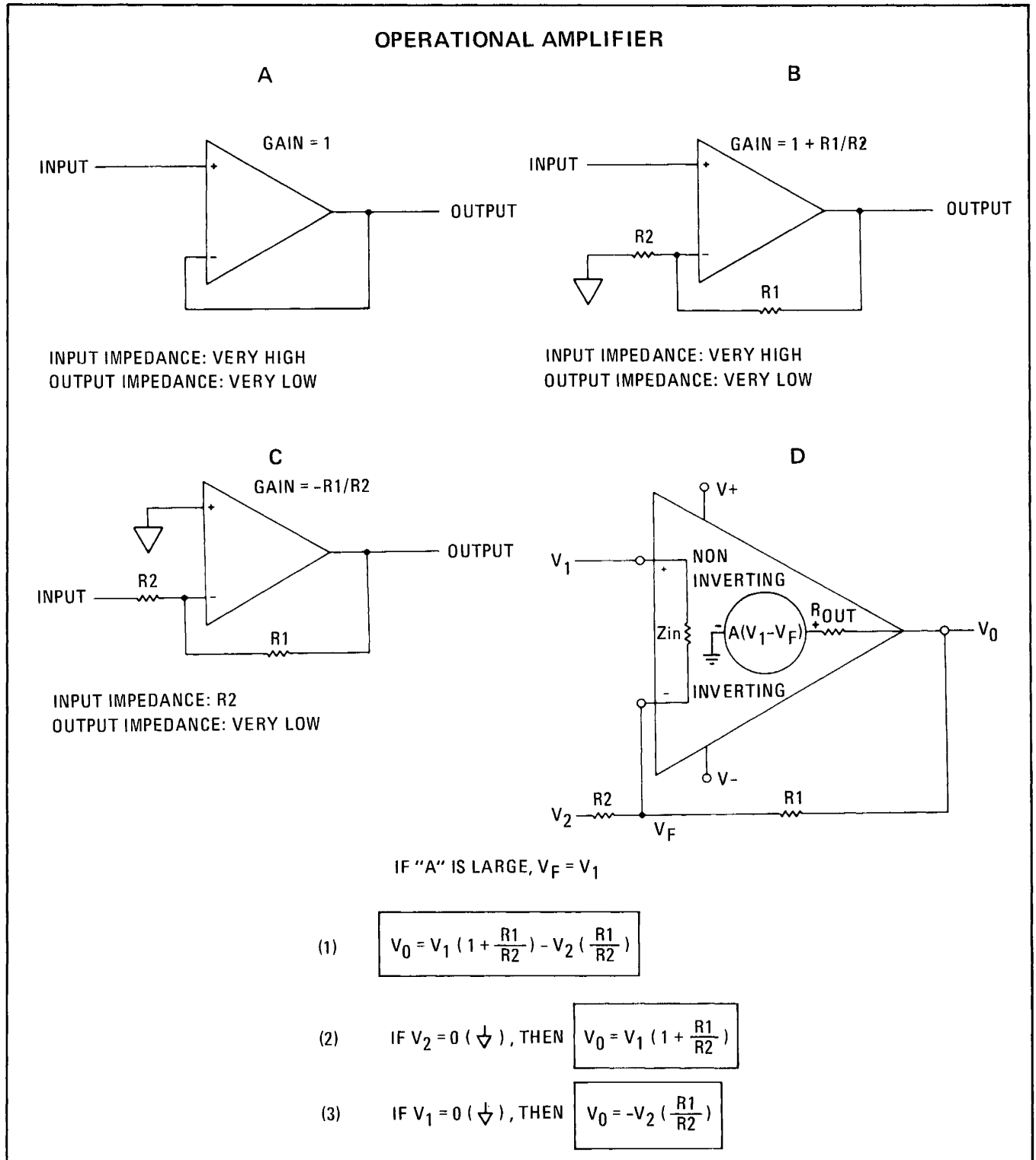
Figure 8-2. Operational Amplifier Equivalent Circuit
