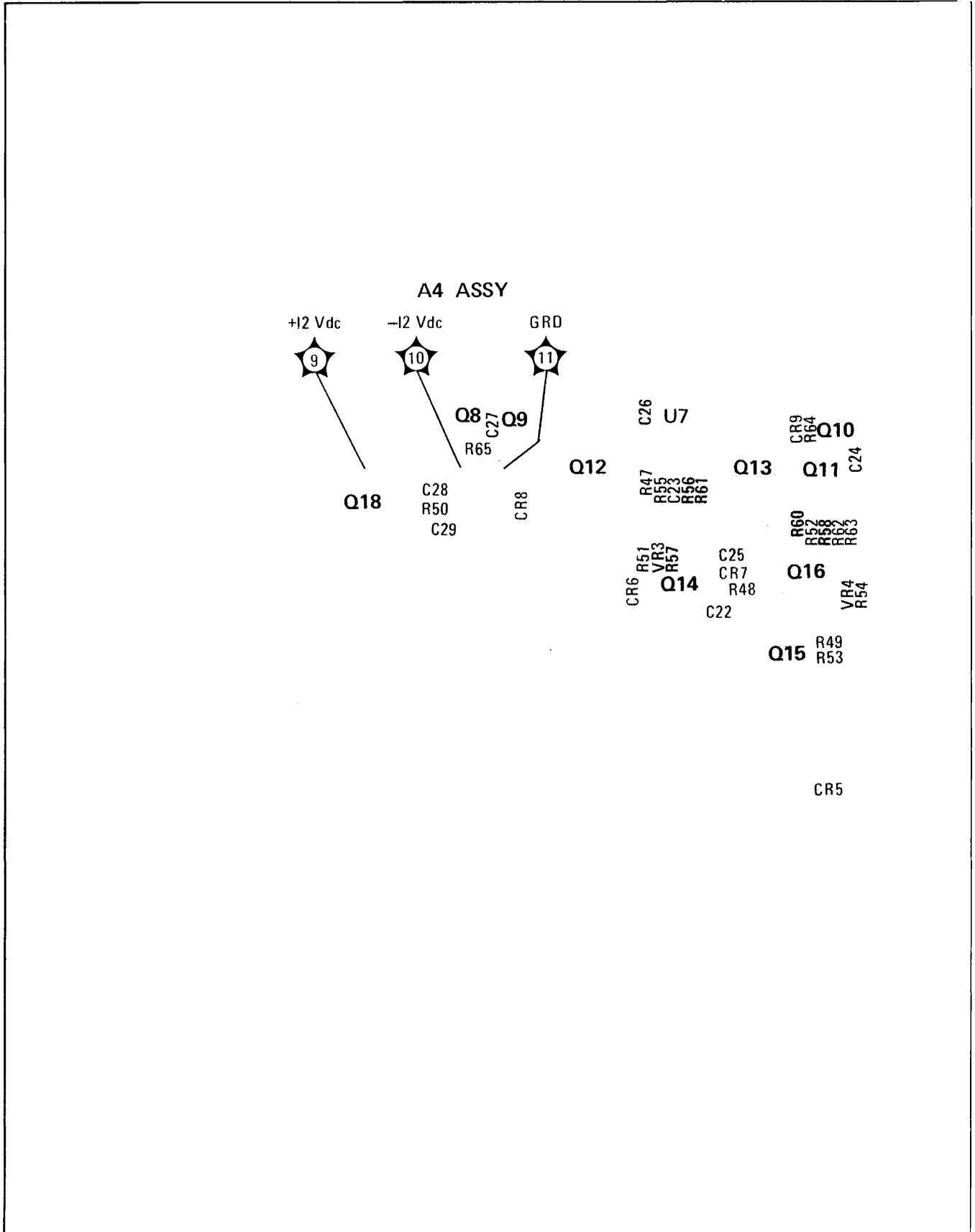
Figure 8-14. P/O A4 Assembly (Power Supply) Component and Test Point Locations
