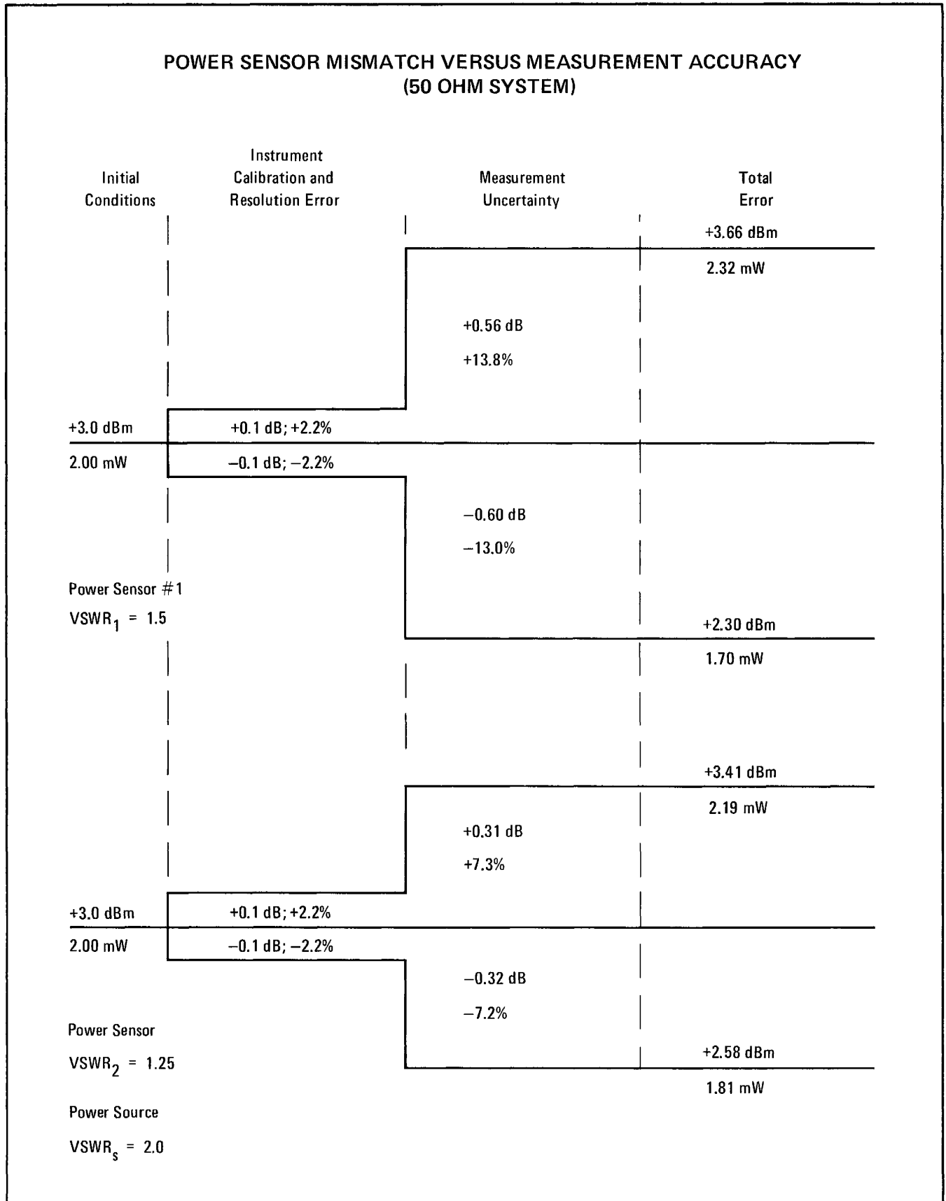
Figure 3-7. The Effect of Power Sensor Mismatch on Measurement Accuracy
