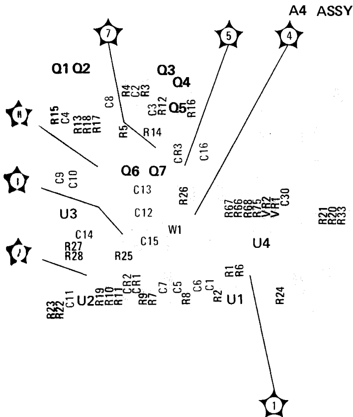
Figure 8-5. P/O A2 Range Switch Assembly (Attenuator) Component Locations
